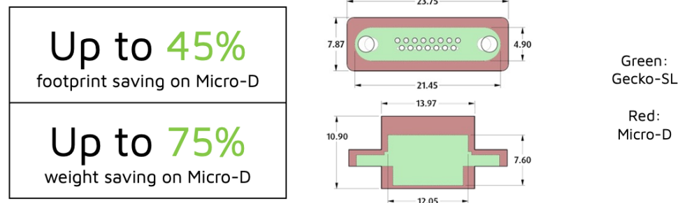
Figure 3: Harwin's Gecko-SL (Screw-Lok) saves up to 45% in connector footprint and up to 75% of connector weight. Image courtesy of Harwin.
